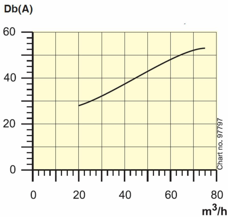
Sound Level Distance to measuring point = 1m
